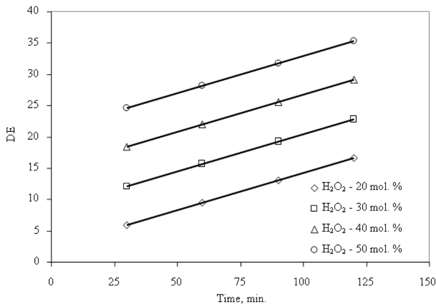
Figure 2 – Effect of time of natural rubber epoxidation at 93 °C on the degree of epoxidation
