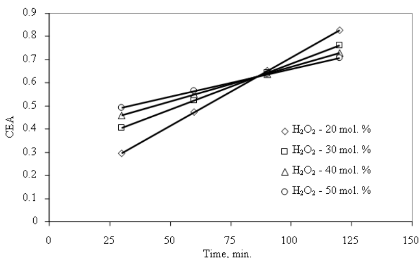
Figure 3 – Effect of time of natural rubber epoxidation at 93 °C on the conversion of epoxidizing agent
