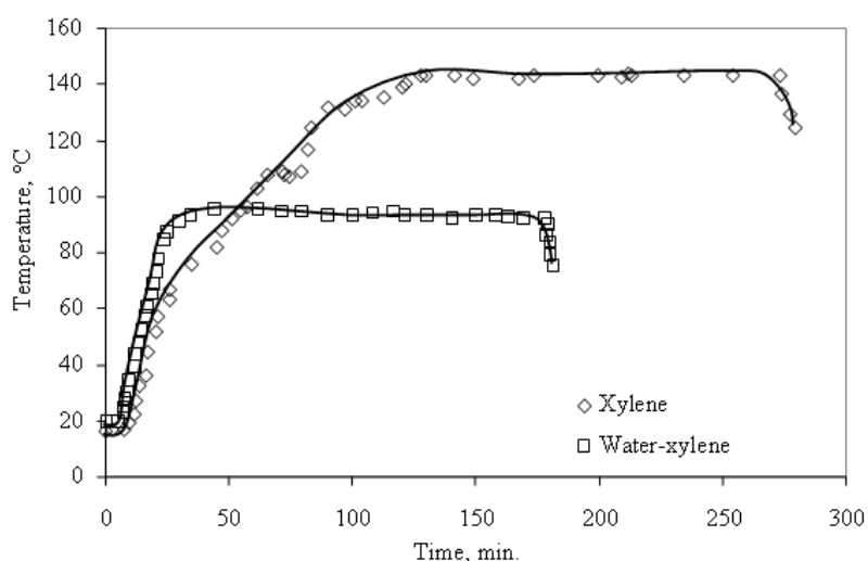
Figure 1 – Thermal regime of natural rubber epoxidation
